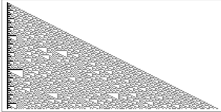
FIGURE 3. Rule 86: a left–right reflected, left-justified image of rule 30, in which the periodicity of columns can be seen. The leftmost sequence of black cells in each row has been highlighted, showing the local nested structure.
