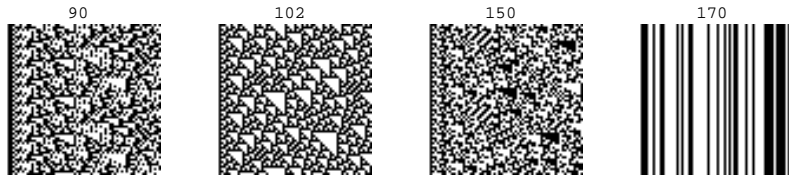
FIGURE 6. The 2-color, range [-2, 0] rules which support white tails and are both right bijective and additive. In the nontrivial cases, the human visual system apparently fails to detect the O(t \log t) computational reducibility of these rules when begun from rightful initial conditions which are not especially simple. The criterion given in Conjecture 3, however, does detect this reducibility.
