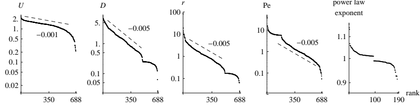
FIGURE 7. The four random walk statistics (drift U , diffusivity D , randomness r , Peclet number Pe ) of the 688 irreducible boundaries decay approximately exponentially when sorted in decreasing order. Dashed lines approximate the slopes on log-linear scales. In the rightmost plot, we sort and plot the exponents of the power law fits for the 190 boundaries deemed to be better fit by a power law ( at^b or at^b + c ) than linear or logarithmic; not shown are the exceptionally small exponents b = 0.03 and 0.01 of rules 7403 and 7419.
